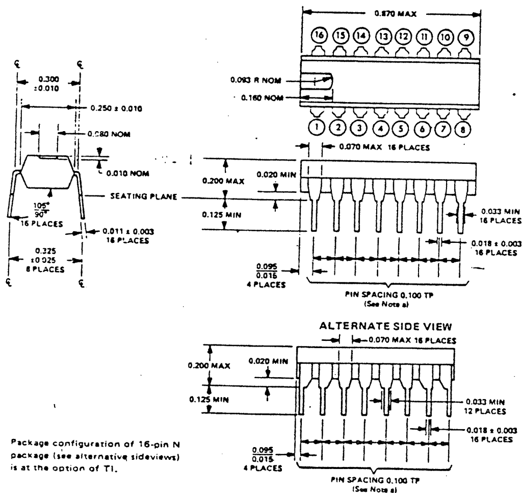
16-PIN N PLASTIC DUAL-IN-LINE PACKAGE OUTLINE
