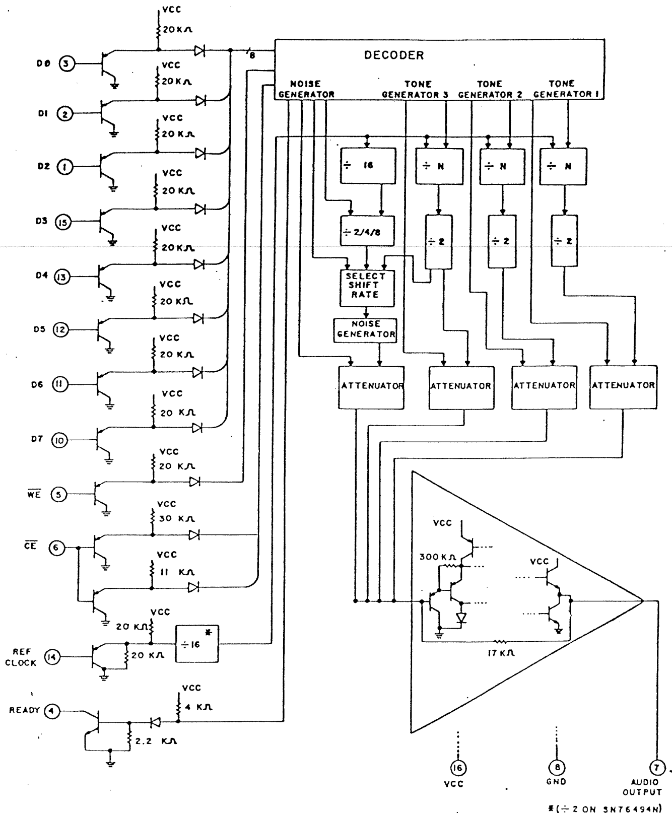
SN76489A / SN76494 SCHEMATIC
