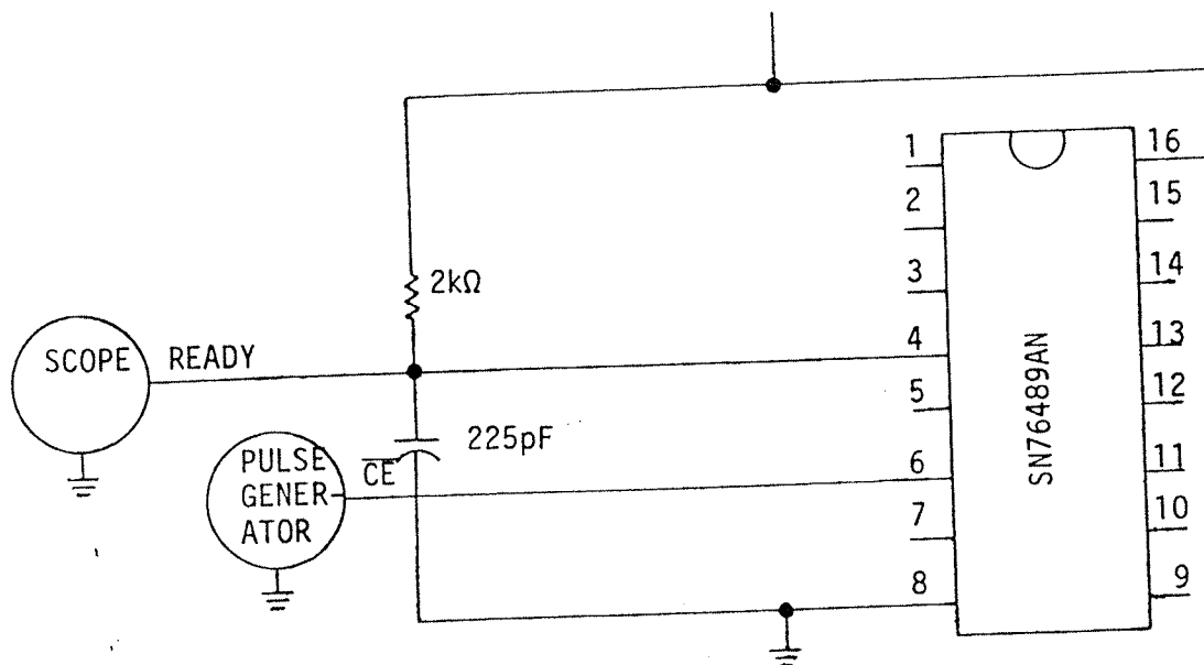
t_{PLL} TEST CIRCUIT
